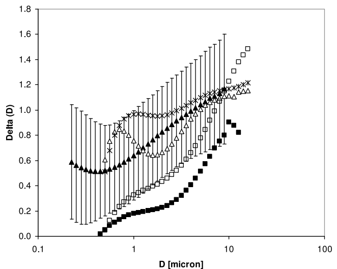
Figure 6. Size distributions of surf-generated aerosols in \delta_{\log}(D) units (see text and equation 4b): solid triangles: onshore flow at Scripps, with standard deviations; solid squares: offshore flow at Scripps; open triangles: onshore flow at FRF; open squares: offshore flow at FRF; asterisks: 3rd offshore event at FRF.
