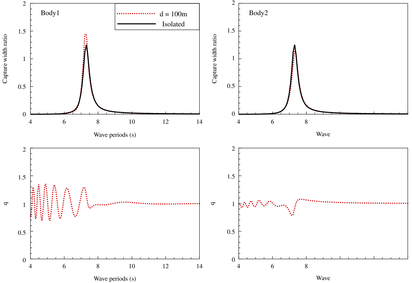
Fig. 6. Capture width ratio and q factors for body 1 (left figures) and body 2 (right figures) of array I in regular waves. The wave direction is 0^\circ and the distance between the two systems is taken equal to 100 m. For the sake of comparison, the capture width ratio of a single isolated system has been plotted too.
