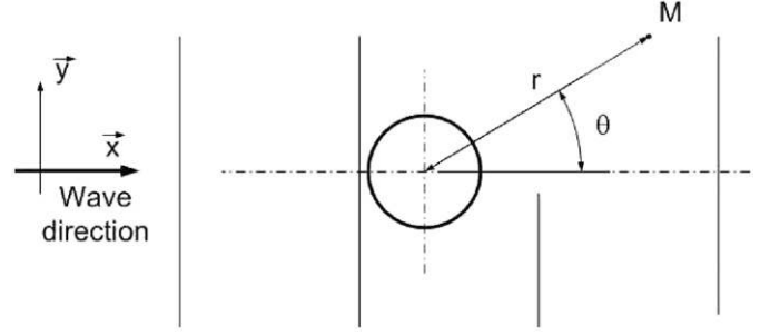
Fig. 18. Notations used for the calculation of wave energy flux far behind a floating system.
