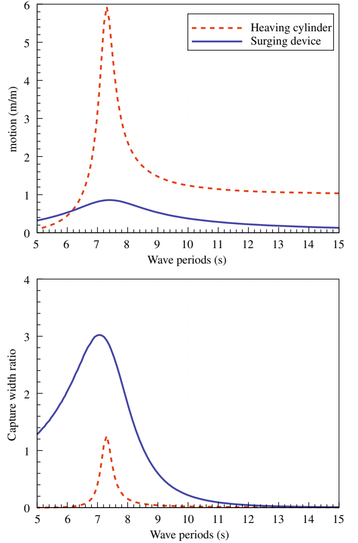
Fig. 5. RAOs (top) and capture width ratio (bottom) of both considered WECs, isolated. Wave direction is 0^\circ .
