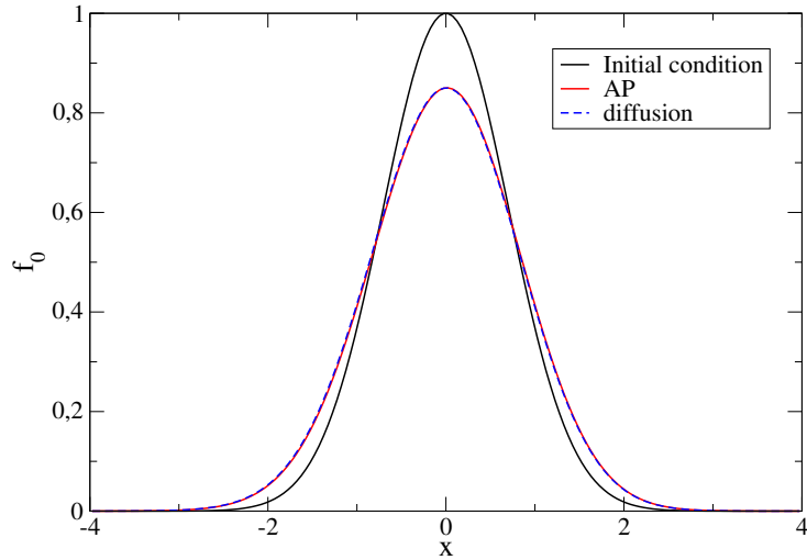
Figure 7: Relaxation of a Gaussian profile in the case of a linear collisionnal parameter: comparison of the f_0 profile for the asymptotic-preserving scheme (AP) and the diffusion solution at time t=150 .
