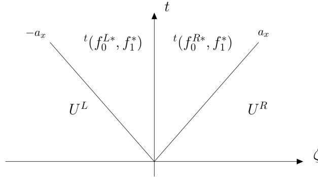
Figure 1: Structure solution of the approximate Riemann problem.
