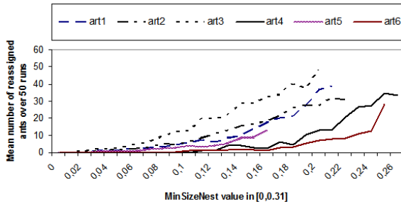
Figure 4: Mean number of reassigned ants versus the values of MinSizeNest \in [0, 0.31] , with Nb_{Meetings} = 20 and Nb_{Learn} = 0.2 * N
