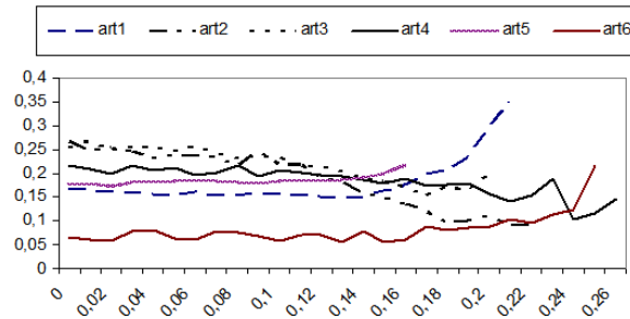
Figure 3: Mean Clustering Error for values of MinSizeNest \in [0, 0.31] , with Nb_{Meetings} = 20 and Nb_{Learn} = 0.2 * N
