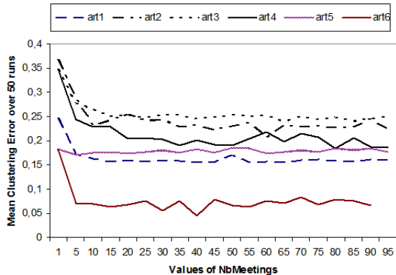
Figure 1: Mean clustering error for values of Nb_{Meetings} \in [1, 95] , with Nb_{Learn} = 0.2 * N and MinSizeNest = 0.05 * N
