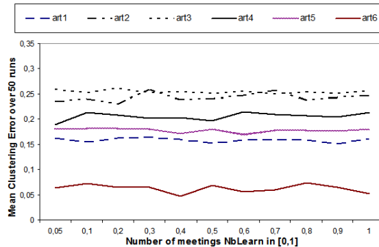
Figure 2: Mean Clustering Error for values of Nb_{Learn} \in [0.05, 1] , with Nb_{Meetings} = 20 and MinSizeNest = 0.05 * N
