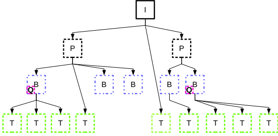
Fig. 6: Initial hypothesis (dashed elements) about the content of a given image I after the initial extractions of panels P , text T and balloons B with tails Q .
