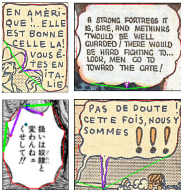
Fig. 24: Result examples of tail tip position and direction detections. Balloon contour hulls are represented in red, hull segments with the two biggest convexity defects in green and detected tails in purple. From top left to bottom right, the detect tail directions are SW, S, E and S.
