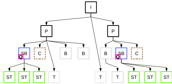
Fig. 9: Hypothesis of ROIs of characters C from the speech balloon SB regions and the corresponding image I . The regions that are not related to ST have been shaded in the graph and removed from the image to make it more comprehensible.
