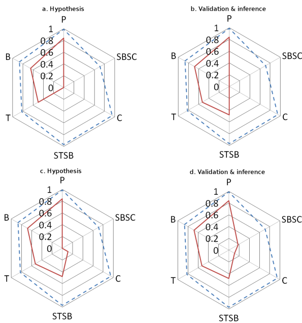
Fig. 26: Evolution of the amount of discovered information for panels P , balloons B , text lines T , comic characters C , STSB and SBSC extractions (solid red line). First and second row correspond to the hypothesis and evaluation steps of the first and second iterations of the process respectively. Values correspond to F-measures for P , B , T , C and accuracies for STSB and SBSC . The dashed blue line represents the best score using our model on the data extracted from the ground truth (optimal condition). The solid red line is the performance of the framework using all the automatic extractions and elements associations presented in this paper.
