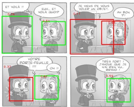
Fig. 25: Example of predicted region (hypothesis of ROI) considered as true (green) or false (red) positives according to the validation criteria a_0 > 0.5 . Thin grey rectangles are the ground truth regions and the red numbers in the top left corner of each ground truth region is the value of the overlapping ratio a_0 . Best viewed in colour.
