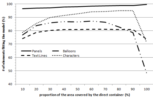
Fig. 5: Percentage of panels, balloons, text lines and characters from the eBDtheque dataset [14] that fit the definition given in 3.2, depending on the area that need to be covered.
