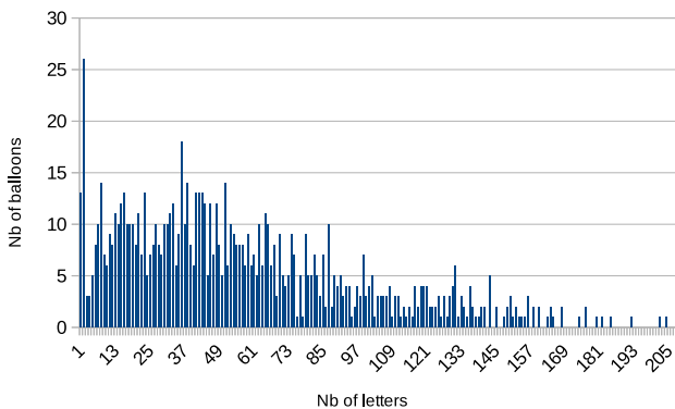
Fig. 23: Distribution of the number of letter per speech balloon.
