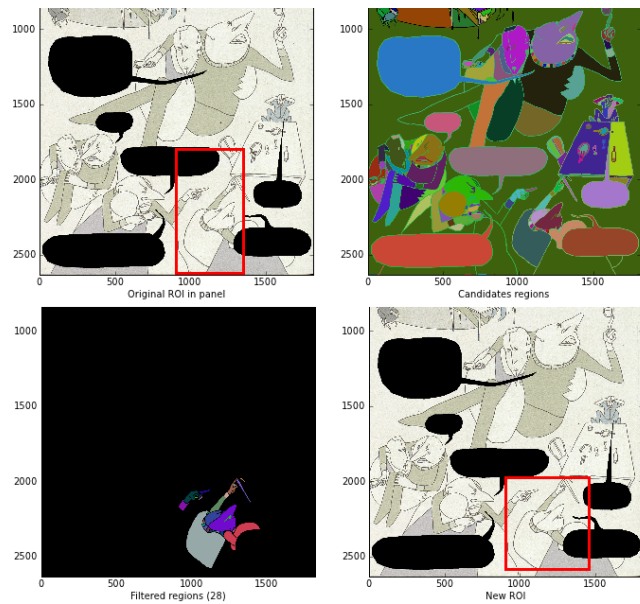
Fig. 20: Hypothetical ROI (red rectangle), region segmentation, region selection and character extraction bounding box (red rectangle) from top-left to bottom-right.
