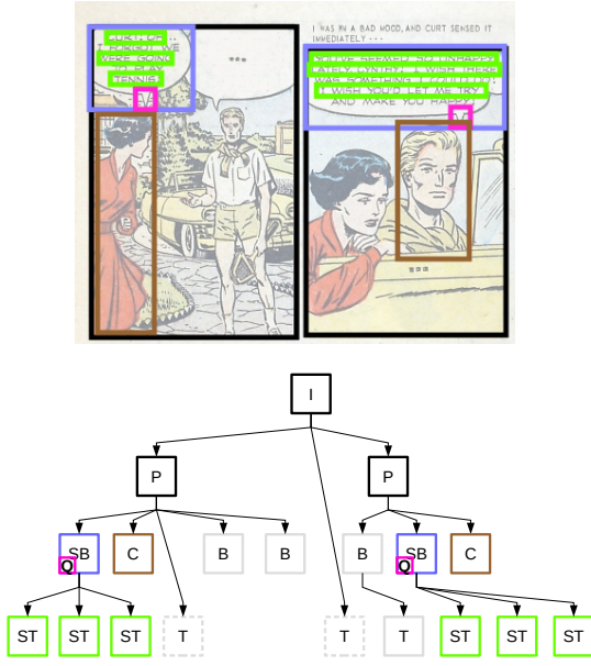
Fig. 11: Validation of the character regions ( C ) by the expert system and the corresponding image I .
