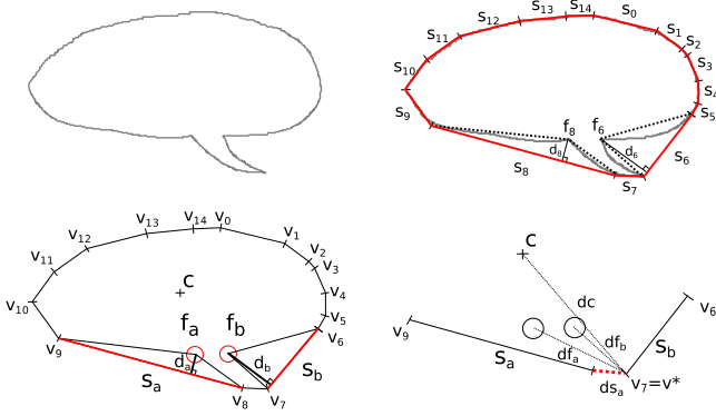
Fig. 17: Convex hull and convexity defects of a speech balloon (top part). Bottom-left figure represents the two biggest convexity defects of depth d_a and d_b which define the tail origin between the two corresponding points on the balloon contour f_a and f_b . Bottom-right figure represents the distances related to the vertex v_7 to illustrate the variables of Equation 3. In this case ds_b = 0 because v_7 coincides with an end of segment s_b (distance equal to zero).
