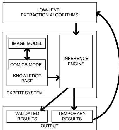
Fig. 3: Generic representation of the expert system and the relationship between knowledge base, the inference engine and the low-level algorithms.
