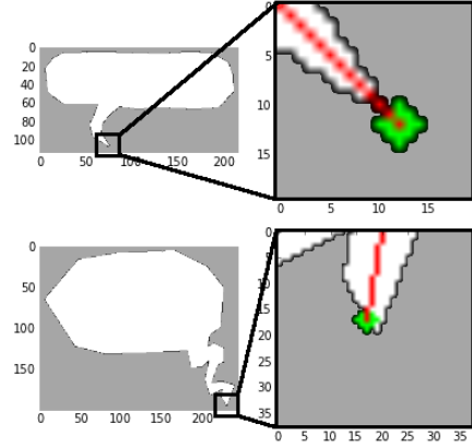
Fig. 18: Tail orientation given by the line fitting algorithm in the neighbourhood of the tail tip. Tail tip is represented as a green square and the result of the fitting algorithm by a red straight line.
