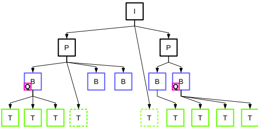
Fig. 7: Validation of the hypothesis using the properties of the knowledge base. Valid elements have a solid border.
