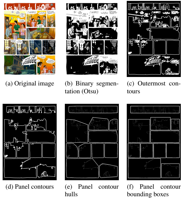
Fig. 13: Panel extraction process.
