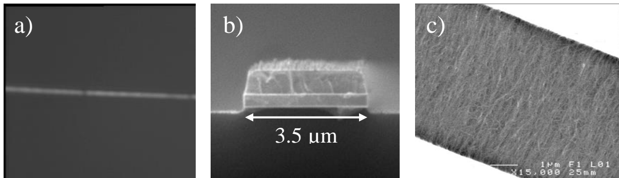
Fig. 2: a) Intensity profile of the planar SWCNT incorporated-waveguide output, b) SEM picture of ridge \text{SiN}_x waveguide with BCB lower cladding (resin was not removed) c) SWCNT aligned by dielectrophoresis between gold electrodes.
