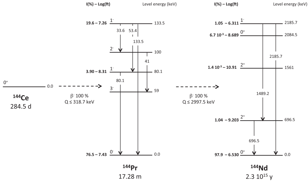
FIG. 1. Simplified decay scheme of the ^{144}\text{Ce} - ^{144}\text{Pr} couple. \beta branches with branching ratios greater than 0.001% are displayed, along with the corresponding Log(ft) values, daughter nucleus level energies and spin parities. The main gamma transitions (intensity greater than 0.1%) among the excited states of the ^{144}\text{Pr} and ^{144}\text{Nd} nuclei are also displayed, together with their corresponding energies. The full ^{144}\text{Ce} and ^{144}\text{Pr} decay scheme data can be found in the National Nuclear Data Center, the Chart of Nuclides database[18].
