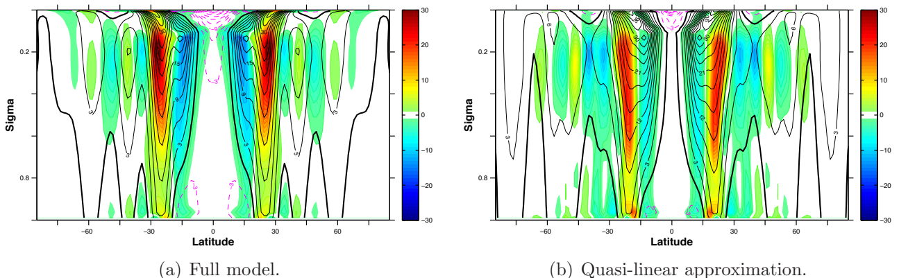
Figure 1. Examples of direct numerical simulations of an atmospheric flow (primitive equations). The colors represent the intensity of the Reynolds' stress divergence (in units 10^{-6}\text{m.s}^{-2} ), and the solid lines are the isolines of the zonally averaged flow (in units \text{m.s}^{-1} ). We clearly see the formation of intense jets (25 \text{m.s}^{-1} ) in high altitudes and midlatitudes ( \sim 30^\circ ). The result of the full simulations (left panel) is in very good agreement with the simulation of the quasi-linear dynamics (right panel), particularly when it comes to the averaged velocity (solid lines). Courtesy Farid Ait Chaalal.
