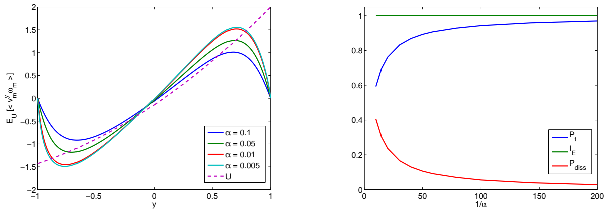
(a) The Reynolds' stress divergence and the zonal flow (dashed line). (b) Stationary energy balance for the fluctuations.
