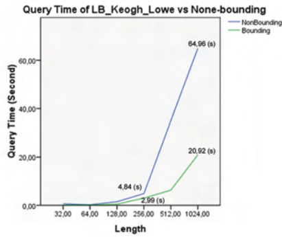
Fig. 15. Comparison the average query time between LB_Keogh_Lowe bounding and none bounding technique
