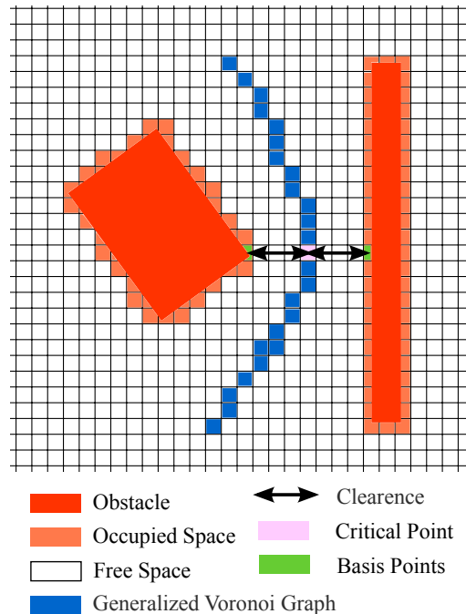
Fig. 4 Sketch of related elements to describe a discretized GVG
