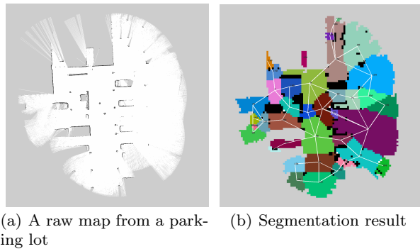
Fig. 1 Topological segmentation of a semi-structured environment. The raw map in (a) covers an area of around 50 \times 50 (m^2) .
