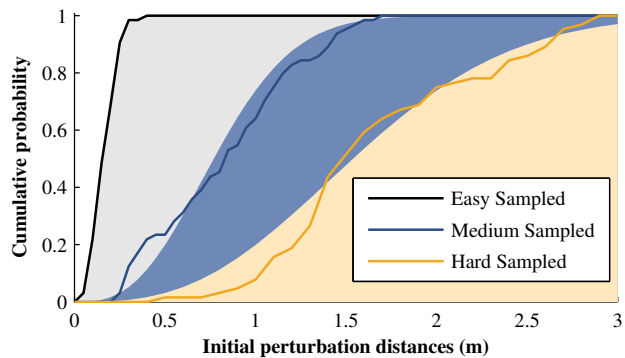
Figure 9 Cumulative probability as function of translation error for each of the perturbation set. The lines are based on the actual 64 samples; the filled backgrounds correspond to the theoretical curves. The easy sampled and theoretical curves overlay due to scaling.
