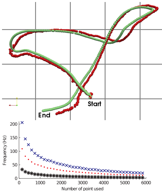
Figure 3 Tracking the pose of a Kinect RGB-D sensor in a home-like environment. Top : projection on the xy -plane of a tracked position (dark-red) versus the measured ground truth (light-green). Each grid square is half a meter. Bottom : performance for different processors: Intel Core i7 Q 820 (blue “x”), Intel Xeon L5335 (red “•”), and Intel Atom Z530 (black “*”).
