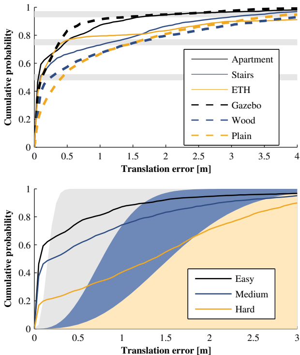
Figure 11 Cumulative probabilities of errors for point-to-plane ICP variant. Top : influence of environments given an easy perturbation level. The gray stripes correspond to the quantiles of interest, namely A50, A75 and A95. Bottom : influence of the three perturbation levels on the Apartment data set with the filled backgrounds correspond to the theoretical curves of initial perturbations.
