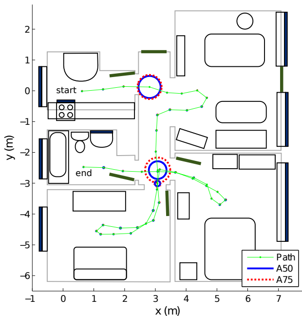
Figure 8 Point-to-plane solution in the Apartment data set: separate statistics for every poses. The path of the scanner (green) with the A50 and A75 statistics overlaid on a sketch of the environment.
