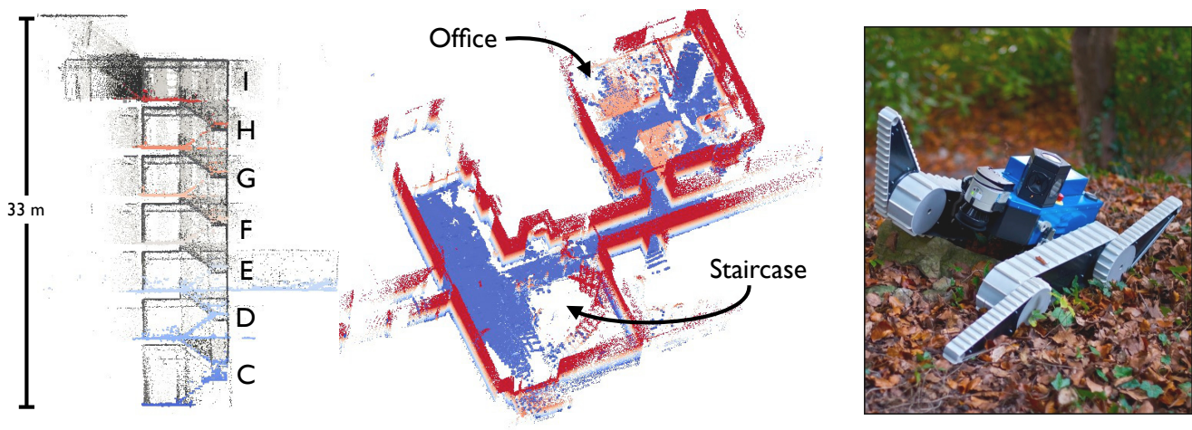
Figure 4 Mapping of a 7-floor staircase using a search-and-rescue robot. Left : side view of the resulting map with the floor colored based on elevation. Middle : top view of the E floor with the ceiling removed and the points colored based on elevation. Right : photograph of the robot with climbing capability.
