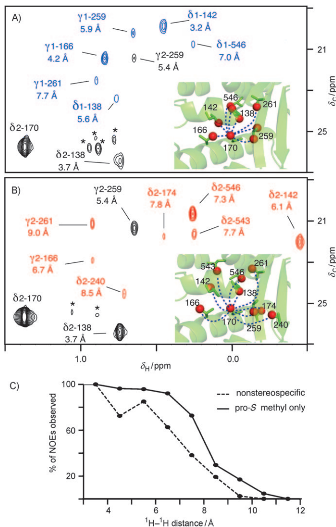
Figure 3. Observation of long-range NOEs between prochiral methyl groups in large proteins. Two-dimensional planes of 4D HMQC–NOESY–HMQC spectra of A) U- ^{12}\text{H} , U- ^{12}\text{C} , Leu/Val- ^{12}\text{C}^2\text{H}_3 , ^{13}\text{C}^1\text{H}_3 and B) U- ^{12}\text{H} , U- ^{12}\text{C} , Leu/Val- ^{13}\text{C}^1\text{H}_3 pro-S MSG samples. Planes were extracted at the F_1 and F_2 frequencies of the \delta_2 methyl group of L170. Observable NOEs involving the \delta_2 methyl group of L170 are labeled. NOE cross-peaks between pro-S and pro-R groups are displayed in blue. NOEs between pro-S methyl groups observed in both spectra are represented in black. New long-range NOEs are displayed in red. All NOEs observed in the 2D plane are shown on the 3D structure of MSG (bottom right in (A) and (B)). The shoulders of diagonal peaks located in adjacent planes are indicated by asterisks. C) Percentage of methyl–methyl NOEs observed relative to those expected, plotted as a function of the inter-methyl ^1\text{H}-^1\text{H} distance. The number of “expected NOEs” corresponds to all pairs of prochiral methyl groups separated by the distance increment with a tolerance of 0.5 Å (i.e. (6.5 \pm 0.5) Å). Inter-methyl distances were derived from the X-ray crystal structure of MSG (PDB code 1d8c). Only distances between pro-S groups were considered for the stereospecifically labeled MSG sample. More detailed information on the methyl–methyl NOEs observed is provided in Figure S6 in the Supporting Information.
