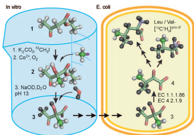
Figure 1. Schematic representation of the production of U-[ ^2\text{H} ], U-[ ^{12}\text{C} ], Leu/Val-[ ^{13}\text{C}^1\text{H}_3 ] ^{\text{pro-S}} proteins. More detailed information on the synthesis is provided in Figure S1 of the Supporting Information. Compound 1: unlabeled ethyl 3-oxobutanoate; 2: ethyl 2-hydroxy-2-[ ^{13}\text{C} ]methyl-3-oxobutanoate; 3: 2-[ ^{13}\text{C} ]methyl-4-[ ^2\text{H}_3 ]acetolactate (or 2-hydroxy-2-[ ^{13}\text{C} ]methyl-3-oxo-4-[ ^2\text{H}_3 ]butanoic acid); 4: ( S )-3-[ ^2\text{H} ]methyl-3-[ ^2\text{H} ]-4-[ ^{13}\text{C} ]- \alpha -ketoisovalerate (or ( S )-2-oxo-3-[ ^2\text{H}_3 ]methyl-3-[ ^2\text{H} ]-4-[ ^{13}\text{C} ]butanoic acid). Products 2 and 3 were produced as a racemic mixture, but only the 2 S stereoisomer of the acetolactate 3 is a substrate of ketol-acid reductoisomerase (EC 1.1.1.86). ^{13}\text{C} , ^2\text{H} , and ^1\text{H} atoms are represented by green, black, and white balls, respectively.
