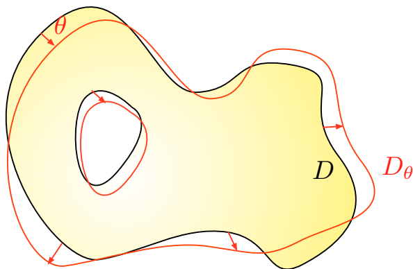
FIGURE 1. One variation D_\theta of a shape D in the framework of Hadamard's method.
