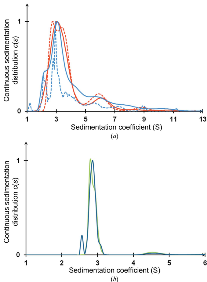
Figure 2 ( a ) Sedimentation curves of ceQORH calculated from absorbance (solid line) and interference (dashed lines) measurements for two ceQORH concentrations: 6 mg ml -1 (red) and 0.6 mg ml -1 (blue). ( b ) Sedimentation curves of ceQORH–NADPH calculated from absorbance (green) and interference (blue) experiments (ceQORH concentration 6 mg ml -1 ; NADPH concentration 1.45 mM).
