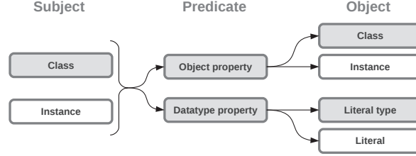
Fig. 2. Constraints on the triples constituting the graph patterns.
