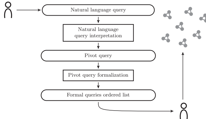
Fig. 1. Overview of the SWIP interpretation process.
