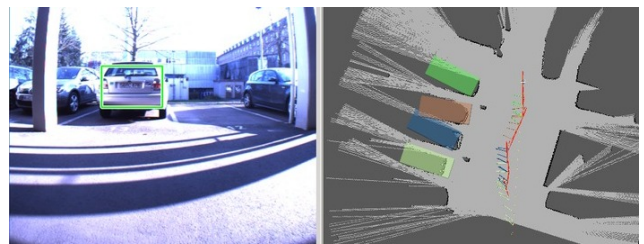
Figure 6: Car detection using visual features. 3D position is computed from multiple detections at different viewpoints, and odometry (red line in 2D map, created by GMapping)
