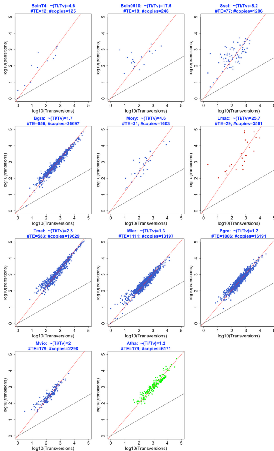
Figure 3 Transition and transversion mutation rates in TE copies from fungal genomes. Transition ( Ti , Y axis, \log_{10} ) and Transversion ( Tv , X axis, \log_{10} ). Mutation rates were calculated using RIPCAL by comparing each TE copy with the TE consensus sequence or the genomic copy with the highest GC content through multiple alignments. Each dot corresponds to the \log_{10}(\text{sum } Ti) vs. \log_{10}(\text{sum } Tv) of a TE family. \sim(Ti/Tv) is the mean of Ti/Tv for all the families in the analysis. The black line corresponds to the linear regression between the two series ( Ti vs Tv ). The red line corresponds to an equiprobable mutation rate ( Ti/Tv = 0.5 ). The Lmac and Atha dot plots are red and green respectively to highlight the pattern of positive and negative controls respectively.
