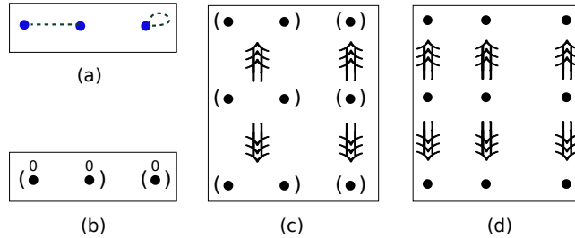
Figure 18: (a) a 0-gmap, (b) its corresponding cellular quasi-manifold, (c) homological equivalences related to the connected components, (d) homological equivalences related to the cells.
