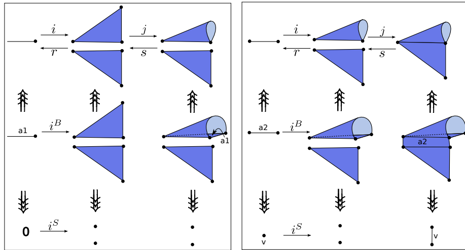
Figure 9: Incremental computation of homological equivalences
