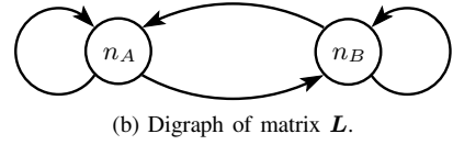
Fig. 5: Equivalence between the circuit diagram and the digraph of the application matrix \mathbf{L} . Some authors call this the dependency graph [10].
