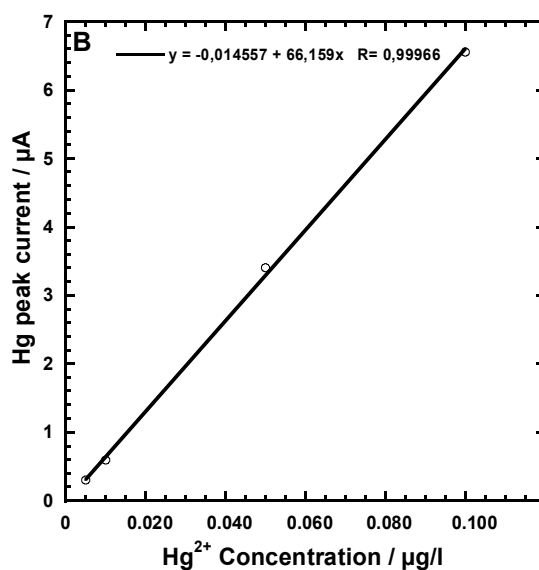
Figure 12: Calibration plot of peak currents at +0.500 V versus Hg^{2+} concentration for the SW-ASV curves in a 10 mM NaCl/ 10 mM HNO_3 electrolyte solution.
