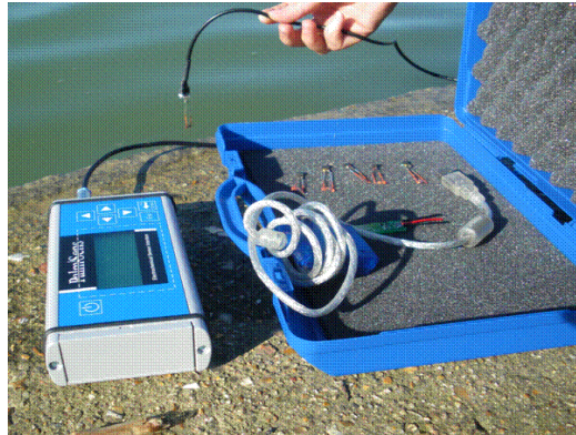
Figure 1. Prototype photograph directly immersed in a natural water.
