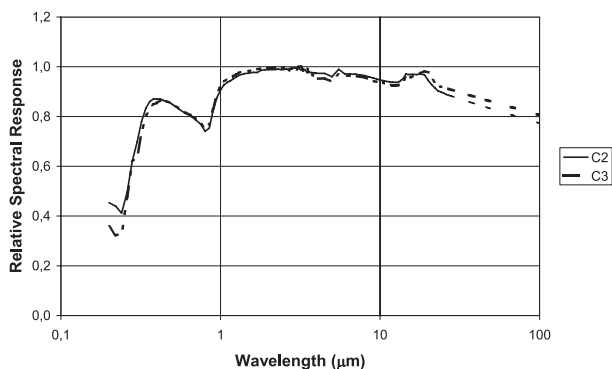
FIG. 3. Relative spectral responses of total channels 2 and 3 of ScaRaB-3/MT.
