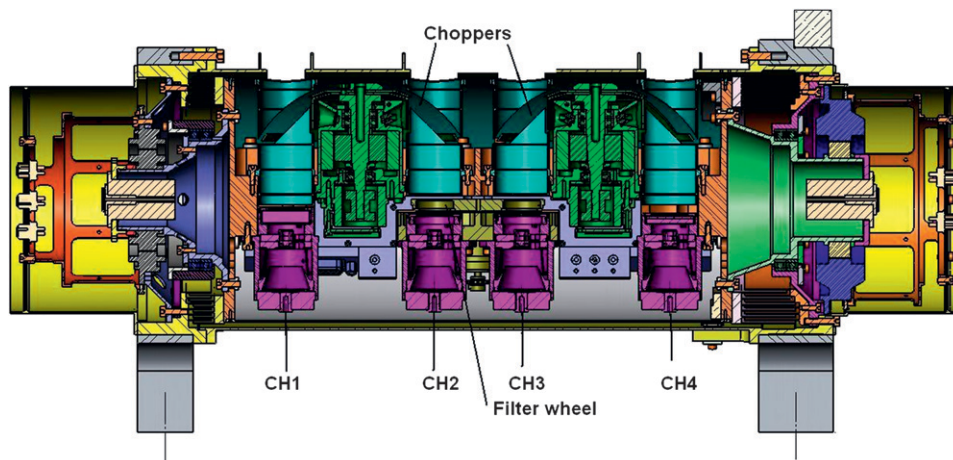
FIG. 1. The ScaRaB rotor. The instrument is organized around two choppers, one for channels 1 (VIS) and 2 (SW) and the other for channels 3 (T) and 4 (IRW).
