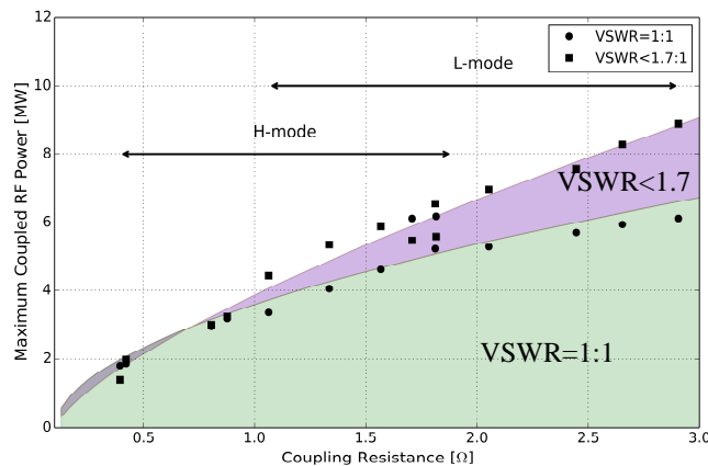
FIGURE 1. Maximum coupled power versus coupling resistance for two matching strategies calculated from the circuit model. Curves correspond to points best fit.
