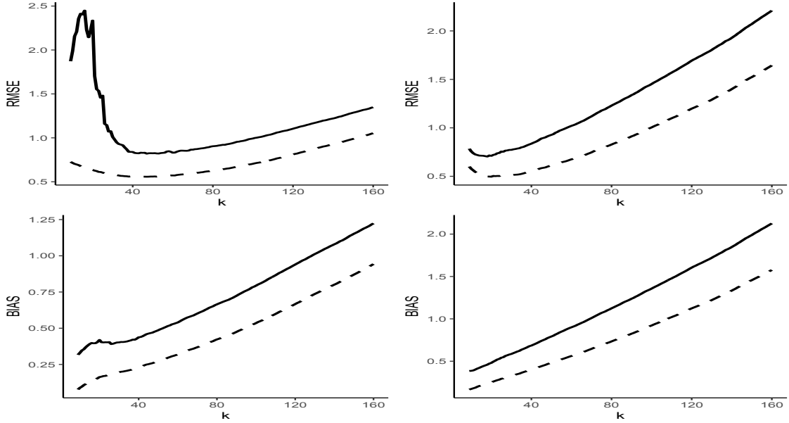
Figure 5: Root MSE estimates (top panels) and Bias estimates (bottom panels) of \widehat{\text{XMES}}^\star/\text{XMES} (solid line) and \widehat{\text{XMES}}^\star/\text{XMES} (dashed line), as functions of k , for the bivariate t_3 and t_5 -distributions on (0, \infty)^2 , respectively, from left to right.
