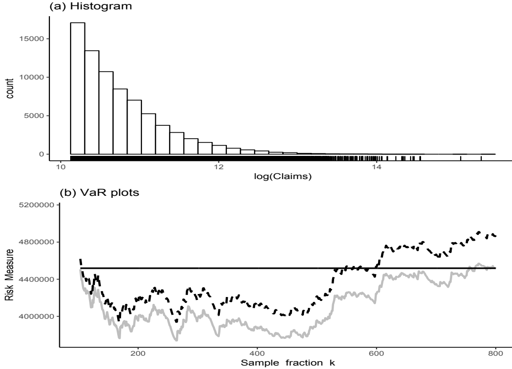
Figure 7: SOA Group Medical Insurance data. (a) Histogram and scatterplot of the log-claim amounts. (b) The VaR plots \{(k, \tilde{\xi}_{\tau'_n(\alpha_n)}^*(k))\}_k in dashed line and \{(k, \hat{q}_{\alpha_n}^*(k))\}_k in solid line, along with the sample maximum Y_{n,n} in horizontal line.
