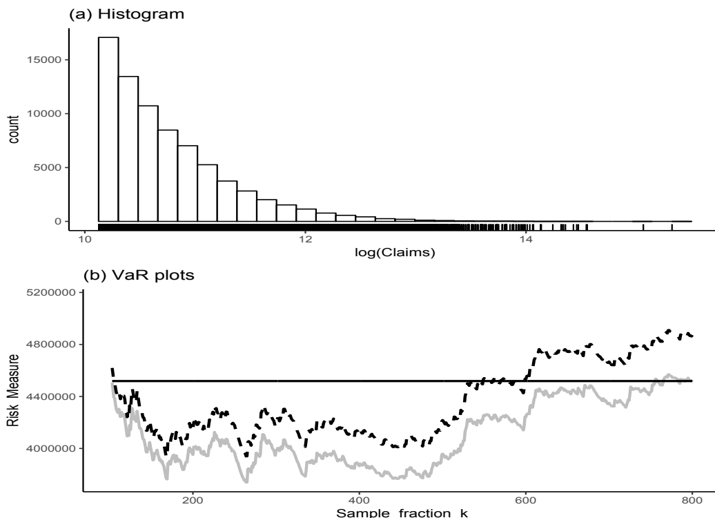
Figure 7: SOA Group Medical Insurance data. (a) Histogram and scatterplot of the log-claim amounts. (b) The VaR plots \{(k, \tilde{\xi}_{\tau_n'(\alpha_n)}^*(k))\}_k in dashed line and \{(k, \hat{q}_{\alpha_n}^*(k))\}_k in solid line, along with the sample maximum Y_{n,n} in horizontal line.
