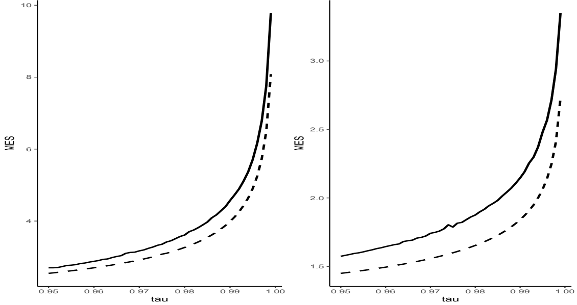
Figure 2: QMES(\tau) in solid line and XMES(\tau) in dashed line, as functions of \tau \in [0.95, 1) . Case of the Student t_\nu -distribution on (0, \infty)^2 . Left: \nu = 3 , right: \nu = 5 .
