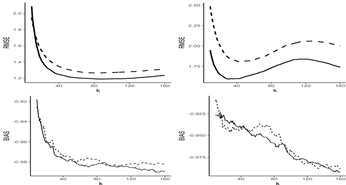
Figure 6: As before—Results for the transformed t_3 and t_5 -distributions on \mathbb{R}^2 .
