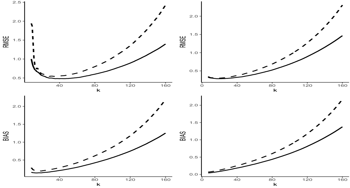
Figure 3: Root MSE estimates (top panels) and Bias estimates (bottom panels) of \tilde{\xi}_{\tau'_n}^*(k)/\xi_{\tau'_n} (solid line) and \hat{\xi}_{\tau_n}^*(k)/\xi_{\tau_n} (dashed line), as functions of k , for the t_3 and t_5 -distributions, respectively, from left to right.
