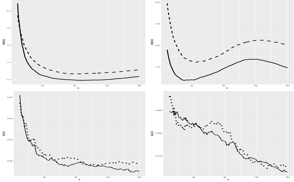
Figure 6: Root MSE estimates (top panels) and Bias estimates (bottom panels) of \widehat{XMESt}^*/XMESt (solid line) and \widehat{XMESt}^*/XMESt (dashed line), as functions of k , for the transformed t_3 and t_5 -distributions on \mathbb{R}^2 , respectively, from left to right.
