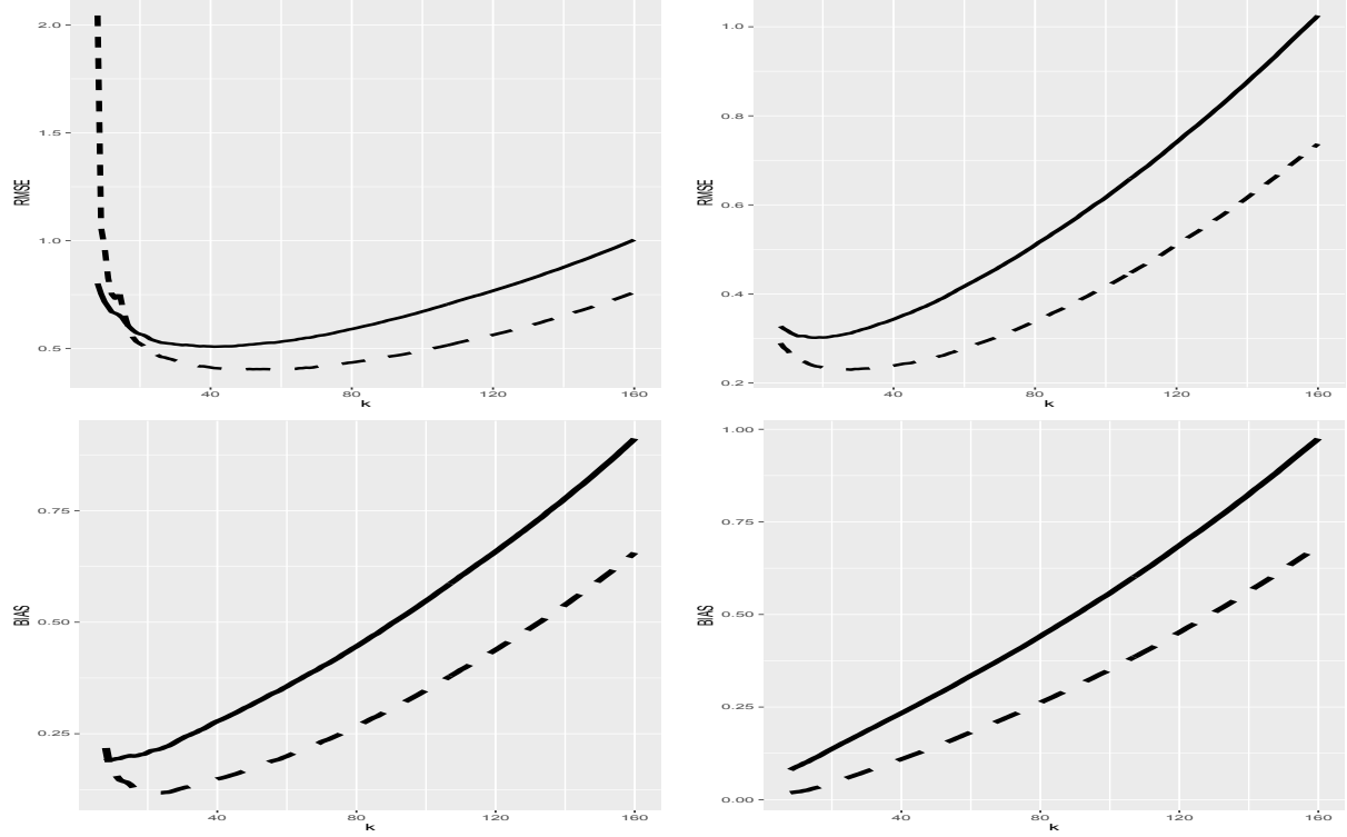
Figure 4: Root MSE estimates (top panels) and Bias estimates (bottom panels) of \tilde{\xi}_{\tau'_n}^*(k)/\xi_{\tau'_n} (solid line) and \hat{\xi}_{\tau'_n}^*(k)/\xi_{\tau'_n} (dashed line), as functions of k , for the truncated Student t_3 and t_5 -distributions, respectively, from left to right.
