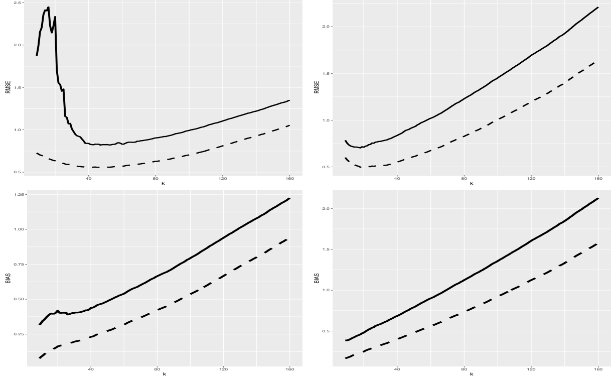
Figure 5: Root MSE estimates (top panels) and Bias estimates (bottom panels) of \widehat{XMESt^*}/XMES (solid line) and \widehat{XMESt^*}/XMES (dashed line), as functions of k , for the bivariate t_3 and t_5 -distributions on (0, \infty)^2 , respectively, from left to right.
