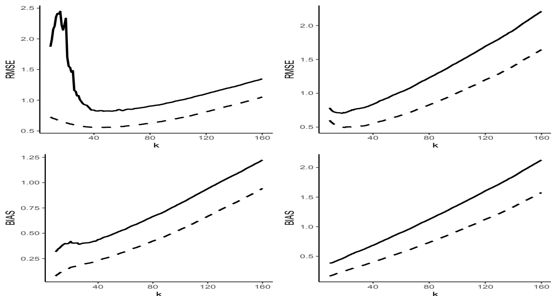
Figure 5 : Root MSE estimates (top panels) and Bias estimates (bottom panels) of \widehat{XMES}^*/XMES (solid line) and \widehat{XMES}^*/XMES (dashed line), as functions of k , for the bivariate t_3 and t_5 -distributions on (0, \infty)^2 , respectively, from left to right.
