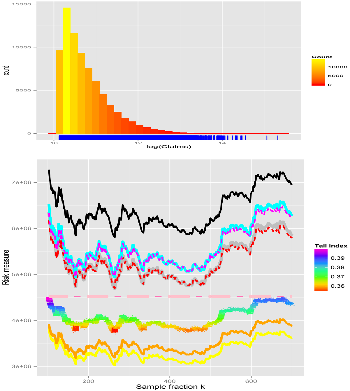
Figure 4: SOA Group Medical Insurance data. (top) Histogram and scatterplot of the log-claim amounts; (bottom) The expectile-based VaR and ES plots \{(k, \hat{\xi}_{1-p_n}^*(k))\}_k in yellow, \{(k, \tilde{\xi}_{1-p_n}^*(k))\}_k in orange, \{(k, \widehat{XES}_k^*(1-p_n))\}_k in gray, \{(k, \widehat{XES}_k^\dagger(1-p_n))\}_k in red, \{(k, \widetilde{XES}_k^*(1-p_n))\}_k in cyan and \{(k, \widetilde{XES}_k^\dagger(1-p_n))\}_k in magenta, along with the quantile-based VaR and ES plots \{(k, \hat{q}_{1-p_n}^*(k))\}_k as rainbow curve and \{(k, \widehat{QES}_k^*(1-p_n))\}_k in black. The sample maximum Y_{n,n} is indicated by the horizontal pink line.
