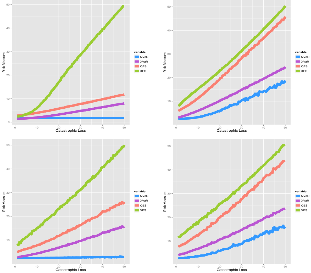
Figure 1: The catastrophic loss sensitivity of empirical quantile-VaR (QVaR), expectile-VaR (XVaR), quantile-ES (QES) and expectile-ES (XES). From left to right and from top to bottom, we have (P, \tau) = (0.01, 0.95), (0.01, 0.99), (0.005, 0.99), (0.005, 0.995) .
