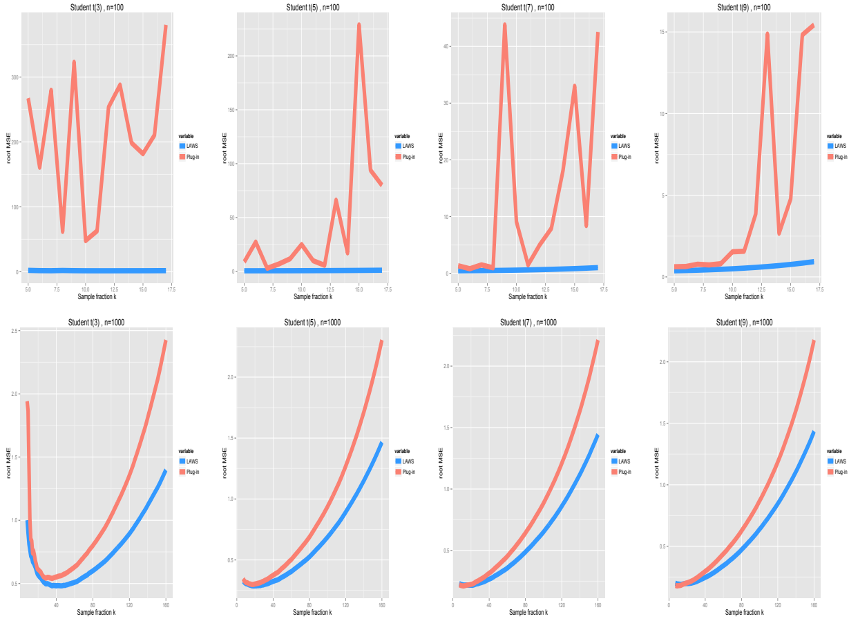
Figure 2: Root MSE estimates for the t_3 , t_5 , t_7 and t_9 -distributions, respectively, from left to right. The sample size n = 100 (top panels) and n = 1000 (bottom panels).
