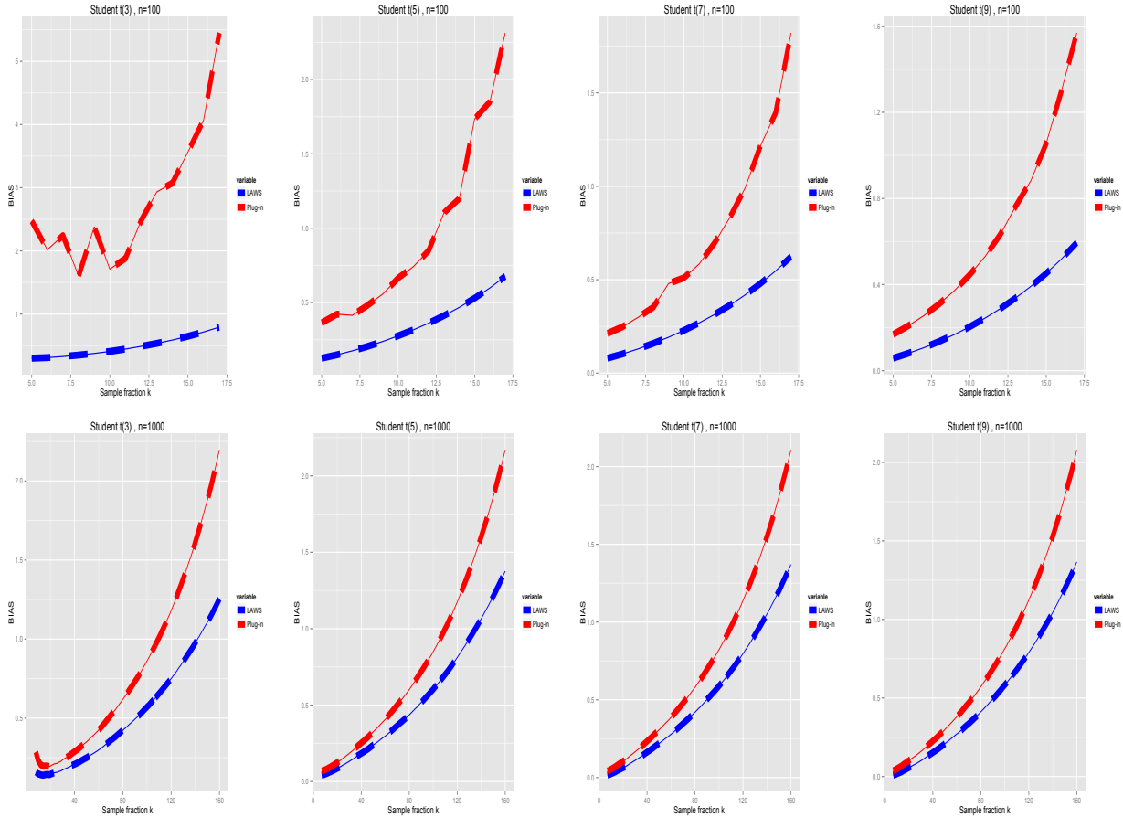
Figure 3: Bias estimates for the t_3 , t_5 , t_7 and t_9 -distributions, respectively, from left to right. The sample size n = 100 (top panels) and n = 1000 (bottom panels).
