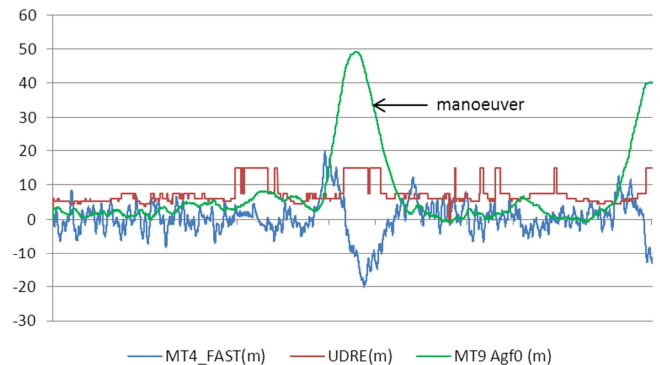
Figure 10: GEO 126 MT4 and MT9 values on 9/01/2012
