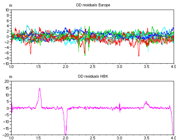
Figure 3: filter residuals for European stations and HBK station, 7-9 January 2012
