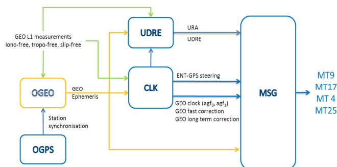
Figure 4: GEO orbit and messages generation processing
