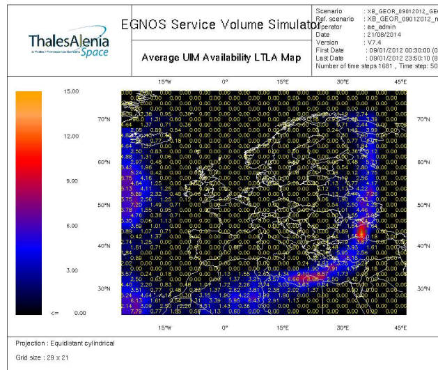
Figure 14: additional APV1 availability percentage provided by GEO126 ranging
