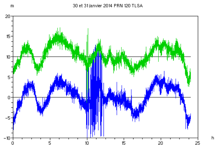
Figure 6: residuals of PRN 120, 30(b) and 31(g) January 2014, Toulouse Station
