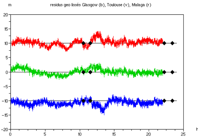
Figure 8: Residuals of GEO 126 on 9/01/2012 with smoothed pseudoranges
