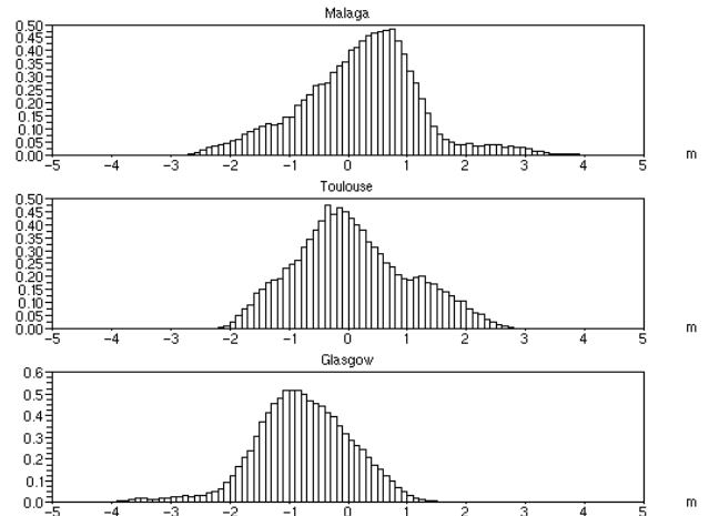
Figure 9: histogram of the residuals
