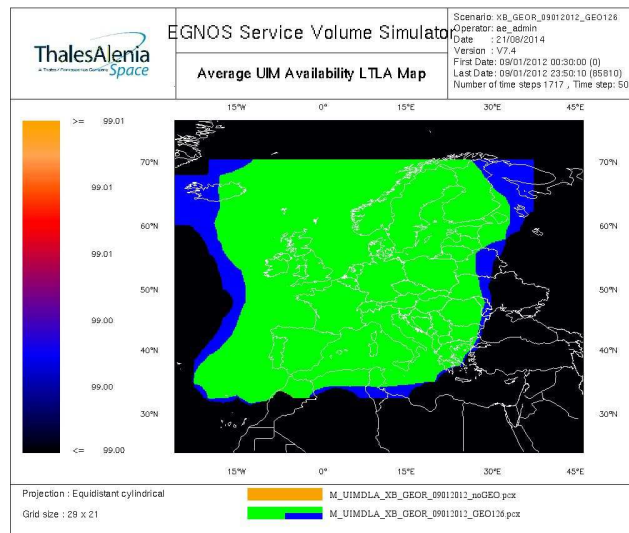
Figure 13: APV1 service area with/without GEO Ranging
