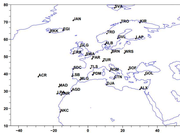
Figure 2: complete EGNOS RIMS network
