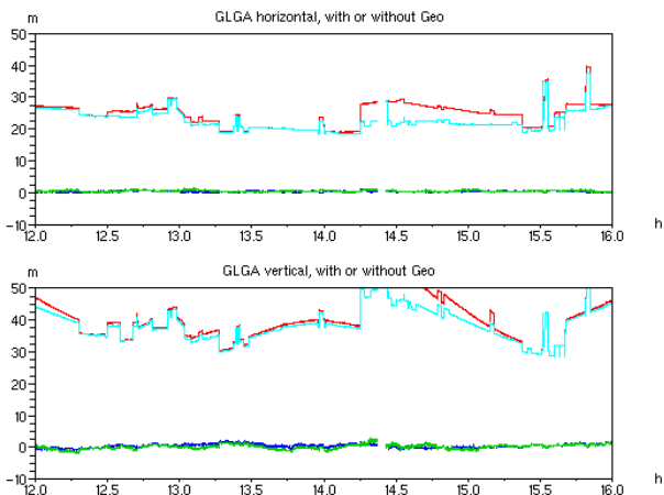
Figure 12: XPE/XPL values for Glasgow station
