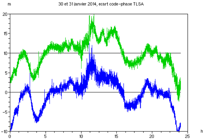
Figure 7: code-phase for PRN 120 in Toulouse, 30 and 31 st January 2014
