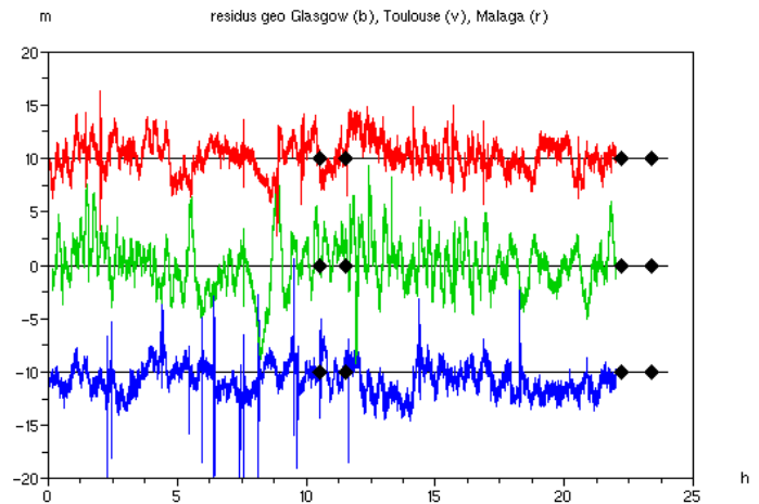
Figure 5: Residuals GEO 126 on 9/01/2012, the symbols correspond to beginning and end of the maneuvers
