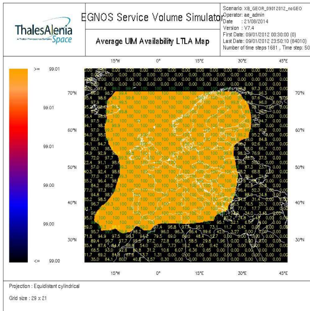
Figure 15: APV1 availability (without GEO Ranging)
