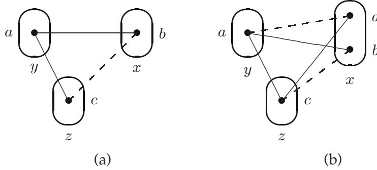
Fig. 5. Illustration of the definition that (a) a variable x is Triangle-supported, (b) a variable x is \exists\forall\text{BTP} -supported
