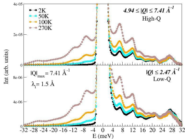
Figure 2. Thermal and Q dependences of the inelastic neutron scattering spectra of \text{CePt}_4\text{Ge}_{12} .
