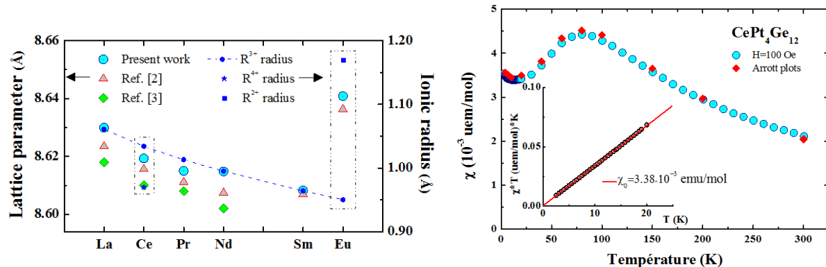
Figure 1. Left: evolution of the lattice parameter in the \text{RPt}_4\text{Ge}_{12} series and comparison with the ionic radii of trivalent R ions (dotted line is a guide for the eyes). The full star represent the ionic radius of \text{Ce}^{4+} and the full square the radius of \text{Eu}^{2+} respectively. Right: thermal evolution of the magnetic susceptibility. In inset the curve \chi.T=f(T) .
