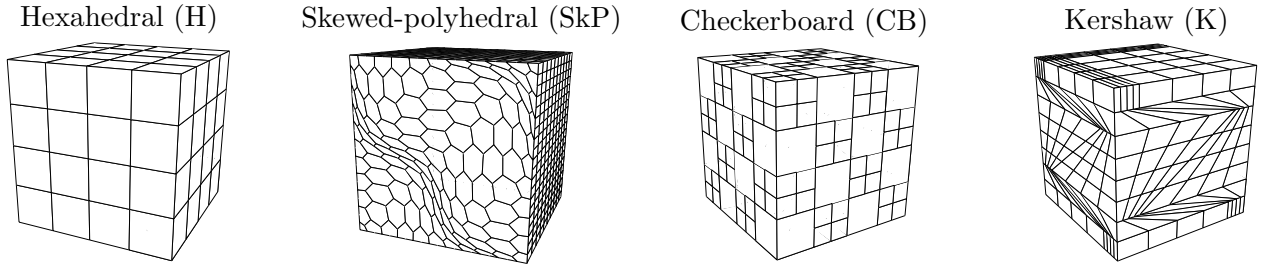
Figure 5: Polyhedral meshes
