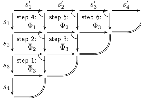
FIGURE 3. Normalising a length- p word in p(p-1)/2 steps, here with p=4 : according to (4.2.4), the six steps correspond to applying \bar{\Phi}_{\delta_4} , that is, \bar{\Phi}_{323123} .
