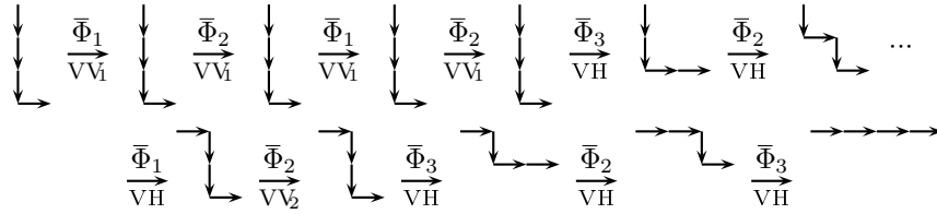
FIGURE 4. Types of the successive steps in the computation of \bar{\Phi}_{12123212323}(w) for w of length 4: in addition to the six VH-steps, which inexorably approach \Phi(w) , we find four VV_1 -steps and one VV_2 -steps; this turns out to be the only possible length-11 sequence for length-4 words.
