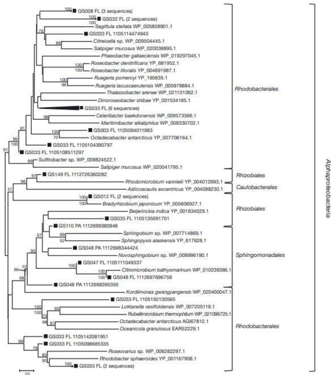
Fig. 2. Phylogenetic tree of annotated and environmental sequences predicted from Global Ocean Sampling (GOS) metaproteome LuxI protein sequences produced using the Neighbour-Joining method with 1000 bootstrap replicates. Only bootstrap support > 50 are shown. Values above branches are those obtained from NJ method; values under branches are those obtained from ML methods. Black squares: environmental sequences; FL: sequences retrieved from free-living fractions; PA: sequences retrieved from particle-attached fractions
