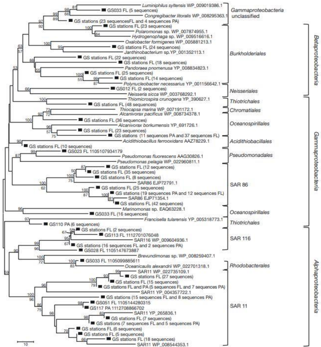
Fig. 3. Phylogenetic tree of annotated and environmental HdtS protein sequences produced using the Neighbour-Joining method with 1000 bootstrap replicates. Only bootstrap support > 50 are shown. Values above branches are those obtained from NJ method; values under branches are those obtained from ML methods. See Fig. 2 for definitions of symbols
