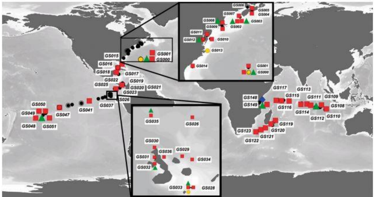
Fig. 1. Geographic distribution of AI-1 (LuxI, HdtS and AinS-like sequences) and AI-2 (LuxS sequences) retrieved from the Global Ocean Sampling (GOS) metagenomes. Black dots: GOS sampling stations where no AI sequences were found; blue diamonds: AinS affiliated sequences; green triangles: LuxI affiliated sequences; red squares: HdtS affiliated sequences; yellow dots: LuxS affiliated environmental sequences. To display the geographic distribution of the environmental sequences related to the 4 different protein families (AinS, LuxI, HdtS and LuxS) a geographic map was built using Ocean Data View software v.4 (ODV Schlitzer, R, Ocean Data View, http://odv.awi.de , 2013)
