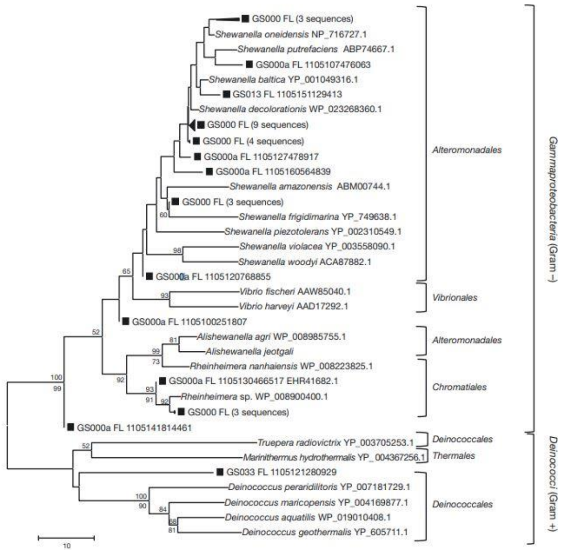
Fig. 4. Phylogenetic tree of annotated and environmental LuxS protein sequences produced using the Neighbour-Joining method with 1000 bootstrap replicates. Only bootstrap support > 50 are shown. Values above branches are those obtained from NJ method; values under branches are those obtained from ML methods. See Fig. 2 for definitions of symbols
