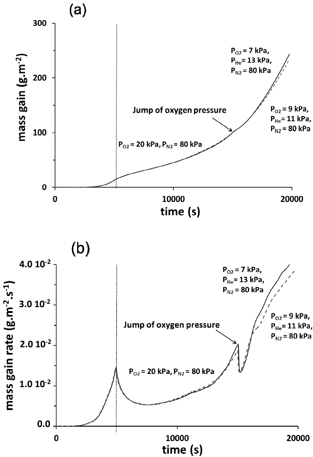
Fig. 5. Jumps of oxygen pressure from 20 kPa to 7 kPa or 9 kPa after 100 \text{ g}\cdot\text{m}^{-2} mass gain at 850^\circ\text{C} . Mass gain curves (a) and mass gain rate curves (b).
