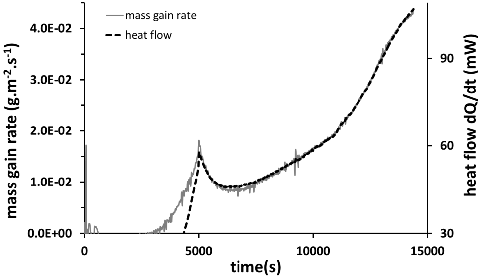
Fig. 3. Mass gain rate (850°C, P_{\text{O}_2} = 20 \text{ kPa} , P_{\text{N}_2} = 80 \text{ kPa} ) and heat flow versus time.
