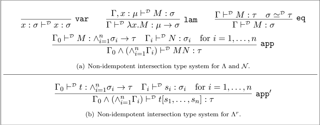
Figure 1: The intersection type systems for \Lambda , \mathcal{N} and \Lambda^r . The other rules for typing \Lambda^r are analogous to (var), (lam), (eq) of Figure 1(a) and are omitted.
