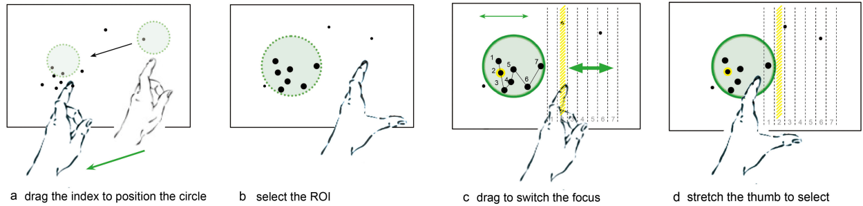
Figure 1: The selection procedures of HorizontalDragger
