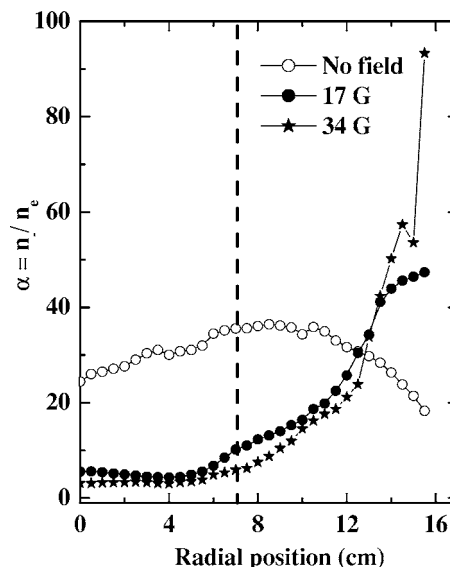
FIG. 6. The radial negative ion fraction dependence on the magnetic field at 1 mTorr and 600 V.
