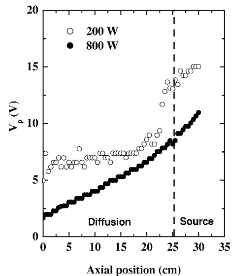
FIG. 4. The axial variation of the plasma potential measured at 1 mTorr and 17 G.
