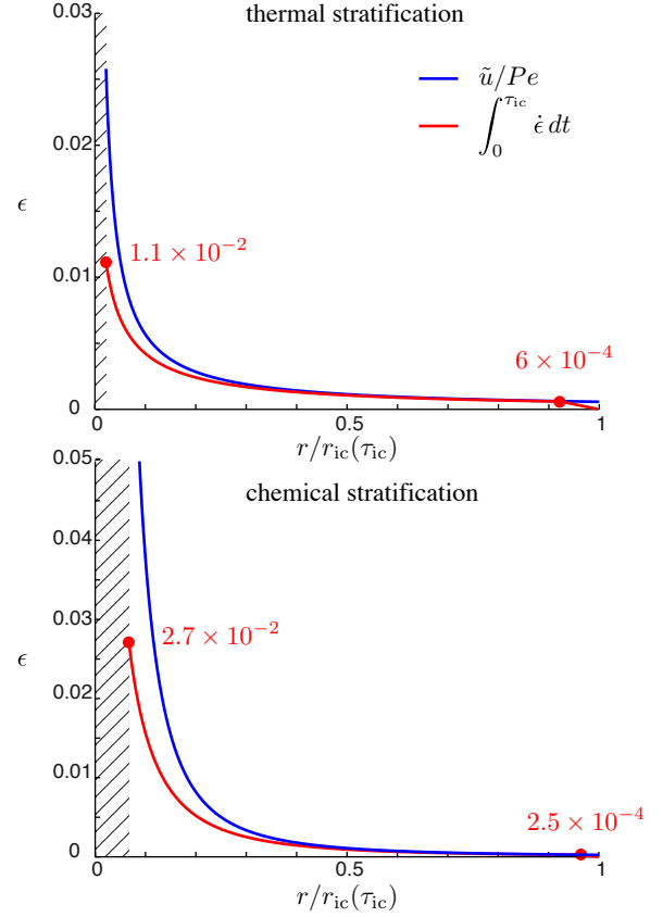
Figure A1. Strain as a function of the radius of the inner core for thermal stratification (a.) and compositional stratification (b.). Integration from equation (E.4) is the red line (analytical solution for thermal stratification and numerical solution for compositional stratification) and the blue lines stand for the estimation u/Pe , which is valid for r > 0.5 r_{ic} . The minimum radius is computed for Ra/M = 1 , limit under which the strong stratification approximation is no longer valid.
