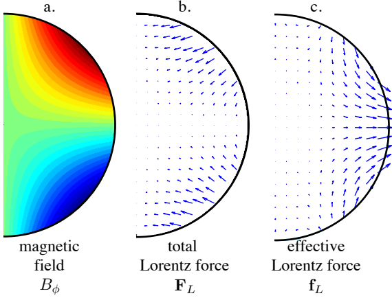
Figure 1. Meridional cross sections showing the intensity of the magnetic field (a), the Lorentz force \mathbf{F}_L (b) and the non-potential part of the Lorentz force \mathbf{f}_L as defined in equation (3) (c).
