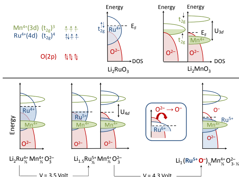
Figure 4. Schematic representations of the density of states (DOS) of \text{Li}_2\text{RuO}_3 , \text{Li}_2\text{MnO}_3 and \text{Li}_{2-x}\text{Ru}_{1/2}\text{Mn}_{1/2}\text{O}_3 in which the Fermi level ( E_F ) is represented by a horizontal dotted line. This figure illustrates the more electronegative character of Ru compared to Mn, the stronger \text{Ru}(4d) - \text{O}(2p) hybridization compared to \text{Mn}(3d) - \text{O}(2p) and the electronic levels involved in the redox processes, i.e. the \text{Ru}^{4+}(t_{2g}) band from x = 2 to 1.5 and the \text{O}(2p) from x = 1.5 to 1.0. Reprinted with permission from 42 (Sathiyaraj, M.; Ramesha, K.; Rousse, G.; Foix, D.; Gonbeau, D.; Prakash, A. S.; Doublet, M. L.; Hemalatha, K.; Tarascon, J.-M. Chem. Mater. 2013 , 25 , 1121). Copyright (2013) American Chemical Society.
