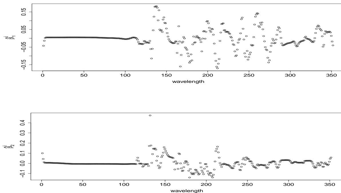
Figure 10: Final first and second EDR directions obtained with SIRs on all the blocks.
