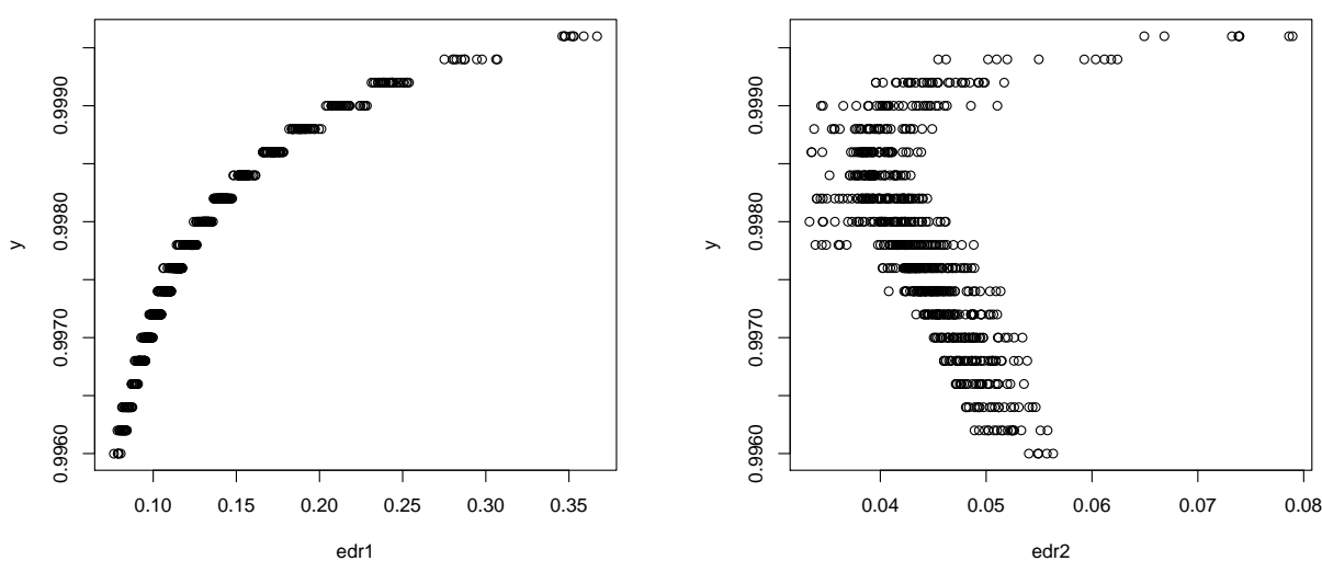
Figure 8: Plots of the dependent variable versus the first EDR index (on the left) and the second EDR index (on the right).
