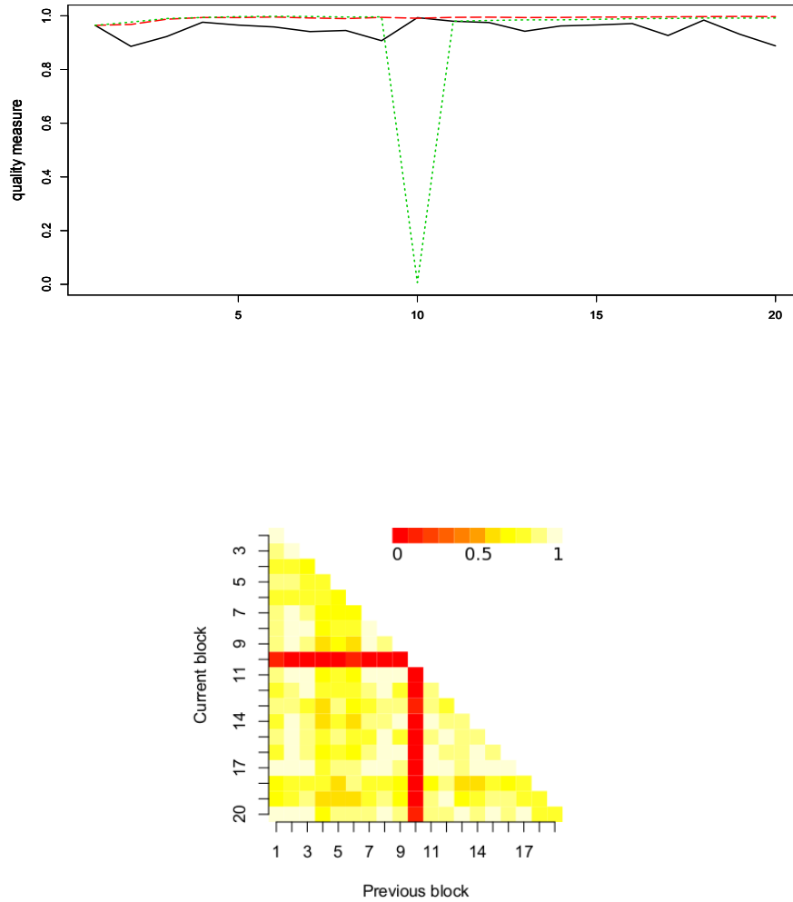
Figure 4: Numerical behavior of the SIRu and SIRds estimators for scenario 1. Top: plot of the quality measure m(\hat{\beta}_t, \beta_t) versus the number t of blocks (dashed red line for SIRds on the first t blocks, dotted green line for SIRu on the first t blocks, solid black line for SIR on block t only). Bottom: image of the weights \cos^2(\hat{\beta}_t, \hat{\beta}_T) used in the computation of the SIRds estimator \hat{v}_T .
