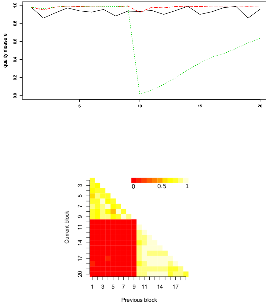
Figure 5: Numerical behavior of the SIRu and SIRds estimators for scenario 2. Top: plot of the quality measure m(\hat{\beta}_t, \beta_t) versus the number T of blocks (dashed red line for SIRds on the first t blocks, dotted green line for SIRu on the first t blocks, solid black line for SIR on block t only). Bottom: image of the weights \cos^2(\hat{b}_t, \hat{b}_T) used in the computation of the SIRds estimator \hat{v}_T .
