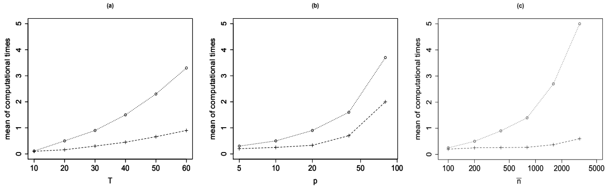
Figure 3: Mean of computational times (in seconds) of sequential SIR ( \circ ) and SIRd ( + ) for various values of T , p and \bar{n} . (a) T \in \{10, 20, 30, 40, 50, 60\} for fixed \bar{n} = 200 and p = 10 . (b) p \in \{5, 10, 20, 40, 80\} (plotted in log-scale) for fixed \bar{n} = 200 and T = 20 . (c) \bar{n} \in \{100, 200, 400, 800, 1600, 3200\} (plotted in log-scale) for fixed T = 20 and p = 10 . For the sake of readability, the points have been joined up with dotted and dashed lines.
