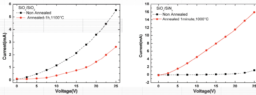
Fig.3. I-V characteristic curves of non annealed and annealed samples (a)SiO x /SiO 2 (b) SiO x /SiN x
