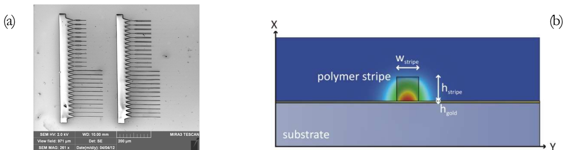
Fig 1. (a) SEM image of a DLSPW series fabricated by e-beam lithography; (b) Cross-sectional view of the DLSPW structure and simulated transverse magnetic field distribution with h_{\text{gold}}=50\text{nm} , h_{\text{stripe}}=600\text{nm} and w_{\text{stripe}}=500\text{nm} .
