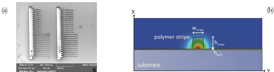
Fig 1. (a) SEM image of a DLSPW series fabricated by e-beam lithography; (b) Cross-sectional view of the DLSPW structure and simulated transverse magnetic field distribution with h_{\text{gold}}=50\text{nm} , h_{\text{stripe}}=600\text{nm} and w_{\text{stripe}}=500\text{nm} .
