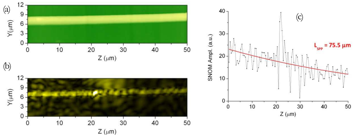
Fig 2. (a) Topography and (b) Optical near-field image on DLSPW; (c) Propagation length L_{\text{SPP}} .
