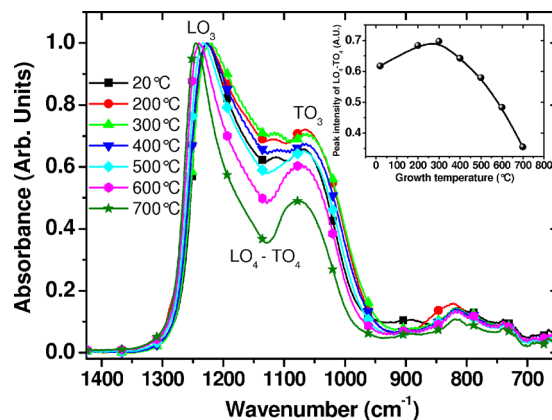
FIG. 2. (Color online) Infrared absorption spectra normalized for as-deposited samples, collected at Brewster angle ( 65^\circ ). Inset: relative evolution of \text{LO}_4\text{-TO}_4 peaks intensity according to the deposition temperature T_d .
